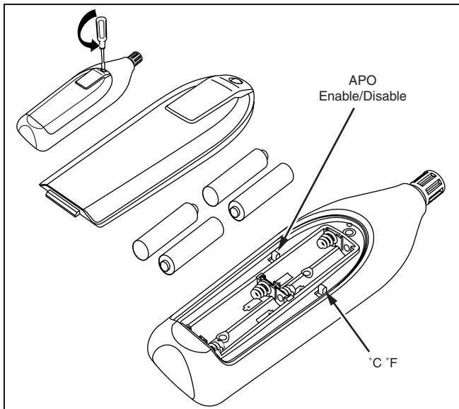
Figure 1. Battery Compartment
